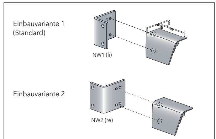
Abb. 18: Montagevariante beachten
